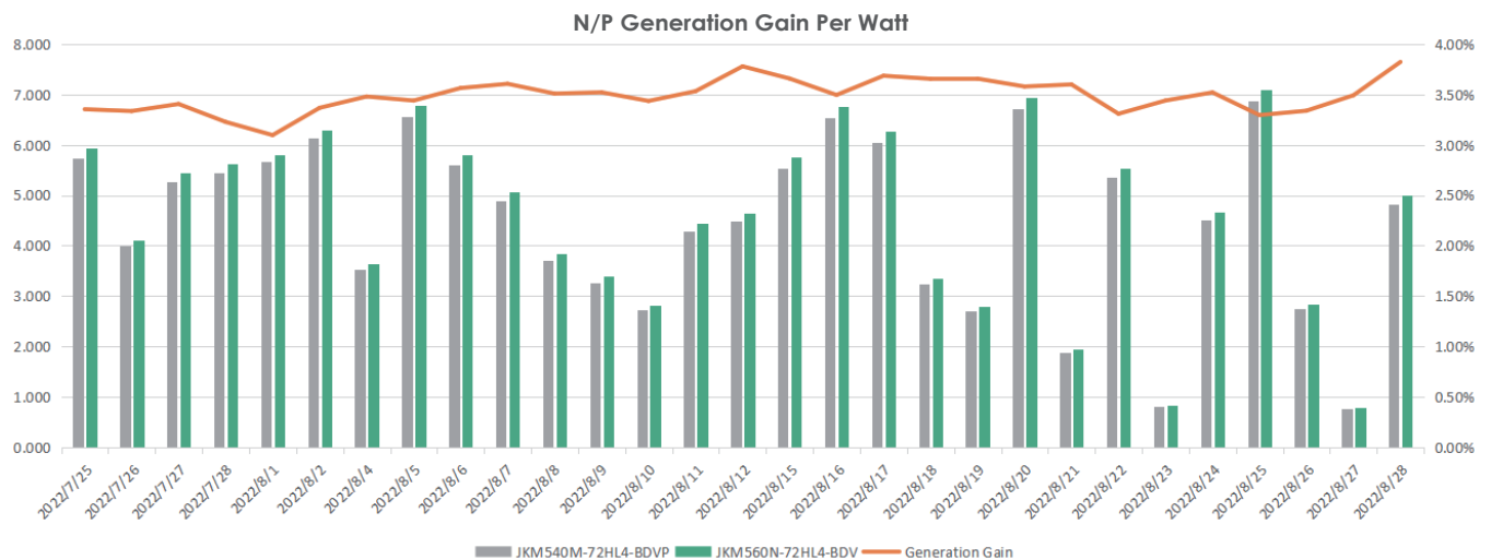
Figure 2. The Difference of Produced Energy in N-TOPCon and P-PERC Bifacial Modules
